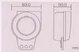
SIGNAL BUZZER
