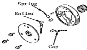
Starter Clutch
